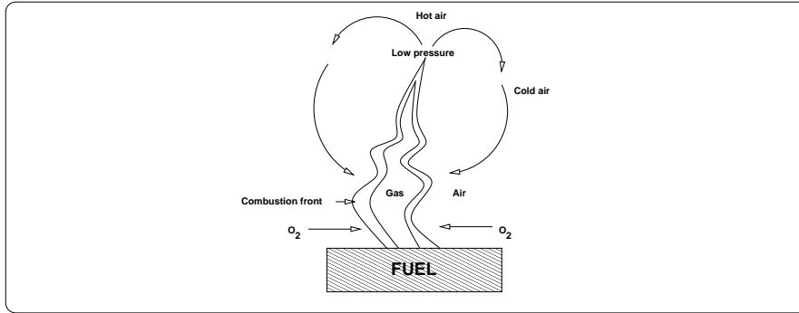
fig 29.1: Flame gas dynamics
